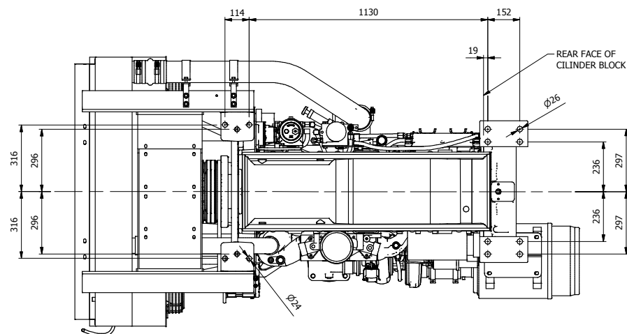
BOTTOM VIEW (CUSTOMER MOUNTING HOLES)
