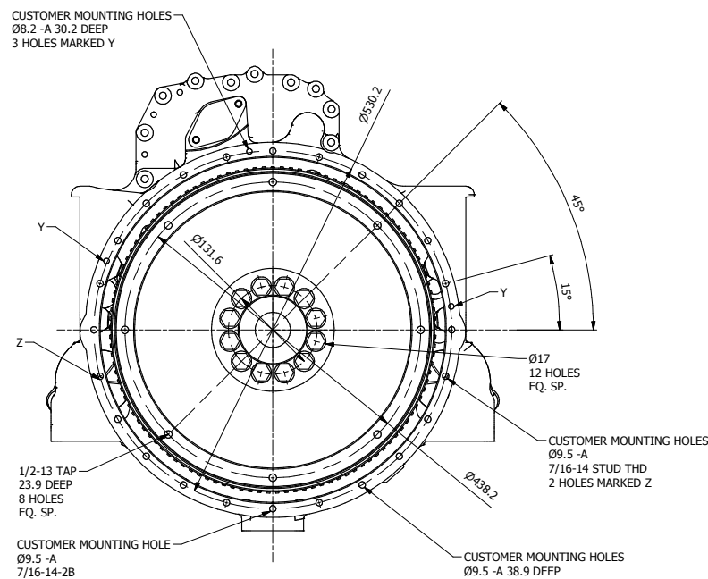
DETAIL FLYWHEEL AND HOUSING ( 1:5 )
